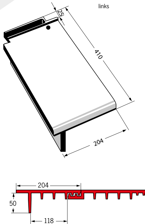
Piano Ortgangziegel
