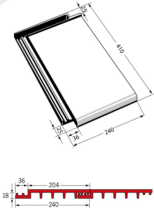
Piano
