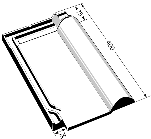
Garant
