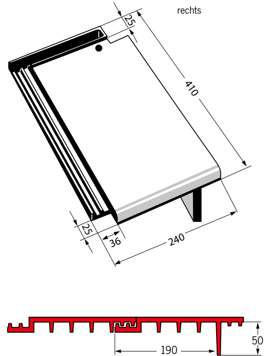
Piano Ortgangziegel
